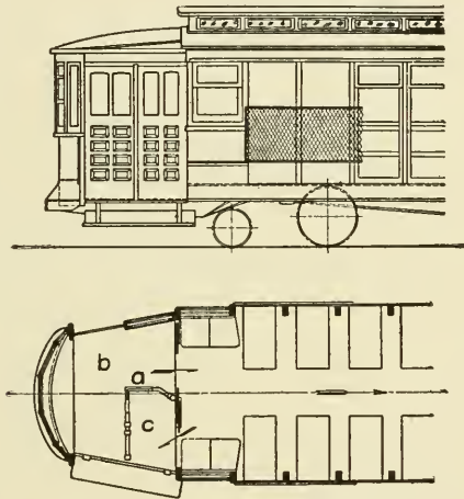
Fig. 8. Pay-as-you-enter Car
